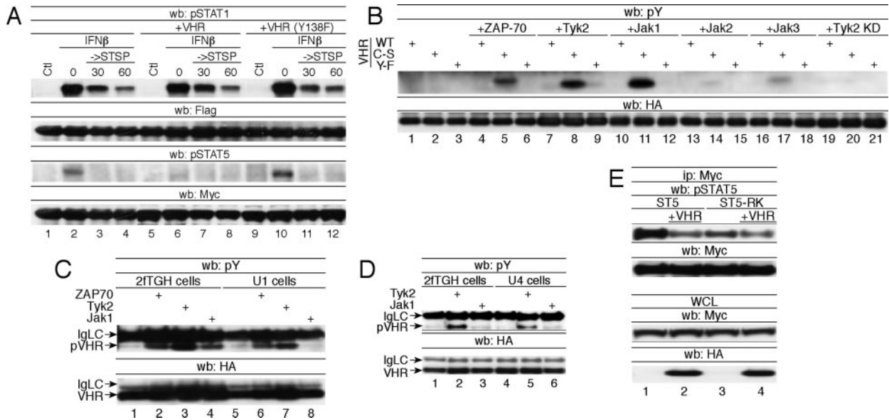
FIGURE 3. Requirement for VHR-Tyr138 phosphorylation as a STAT5 phosphatase. A , 293T cells were transiently transfected with FLAG-STAT1 or Myc-STAT5A and either empty vector or WT VHR, VHR(C→S), or VHR(Y→F). A pulse-chase experiment was performed as described in Fig. 1 A . Tyrosine phosphorylation and efficiency of immunoprecipitation of FLAG-STAT1 and Myc-STAT5A were analyzed using the indicated Abs. B , Cells were transfected with the indicated HA-tagged VHR and kinase constructs and phosphorylation of immunoprecipitated VHR was determined by anti-phosphotyrosine (pY) Western blotting (wb). C , 2fTGH cells and their Tyk2-deficient counterparts (U1) were transfected with HA-VHR(C→S) and the indicated tyrosine kinase. Anti-HA immunoprecipitated VHR was analyzed for its tyrosine phosphorylation ( upper panel ). D , Same as C , except that Jak1-deficient U4 cells were used for transfection. E , Myc-STAT5A or STAT5A(R→K) were cotransfected with Tyk2 and HA-VHR as indicated. Phosphorylation of immunoprecipitated (Ip) STAT5 was determined by anti-phospho-STAT5 (pSTAT5) immunoblotting. IgLC, Ig light chain; STSP, staurosporine; WCL, whole cell lysate.
