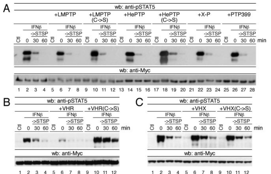
FIGURE 1. Identification of VHR as a STAT5 tyrosine phosphatase. A , 293T cells were transfected with plasmids encoding Myc-STAT5A and either empty vector or the respective WT or catalytically inactive phosphatases as indicated. Forty-eight hours after transfection, cells were left untreated (control (Ctl)) or stimulated with IFN \beta (1000 U/ml) for 60 min before the addition of staurosporine (STSP) at 500 nM, and incubation was continued for the indicated time periods. Tyrosine phosphorylation of immunoprecipitated Myc-STAT5A was analyzed by using anti-phospho-STAT5 (upper panel) and anti-Myc Abs (lower panel). B and C , Same as in A , except that cells were transfected with Myc-STAT5 and empty vector or HA-tagged VHR or VHX. wb, Western blotting; LMPTP, low m.w. PTP, HePTP, hemopoietic PTP.
