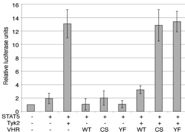
FIGURE 4. Inhibition of STAT5-mediated transcription by VHR. 293T cells were transfected with the indicated plasmids and the STAT5-responsive \beta -casein-luciferase. CMV-driven \beta -galactosidase was included to normalize for transfection efficiency. Cells were lysed 48 h after transfection, and lysates were analyzed for luciferase and \beta -galactosidase activity. Average results of four independent experiments are shown. CS, C→S; YF, Y→F.
